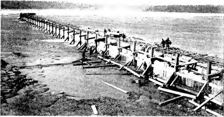
WING DAM OF ONE OF THE CANADIAN COMPANIES RUNNING OUT TO THE EDGE OF THE RAPIDS.
